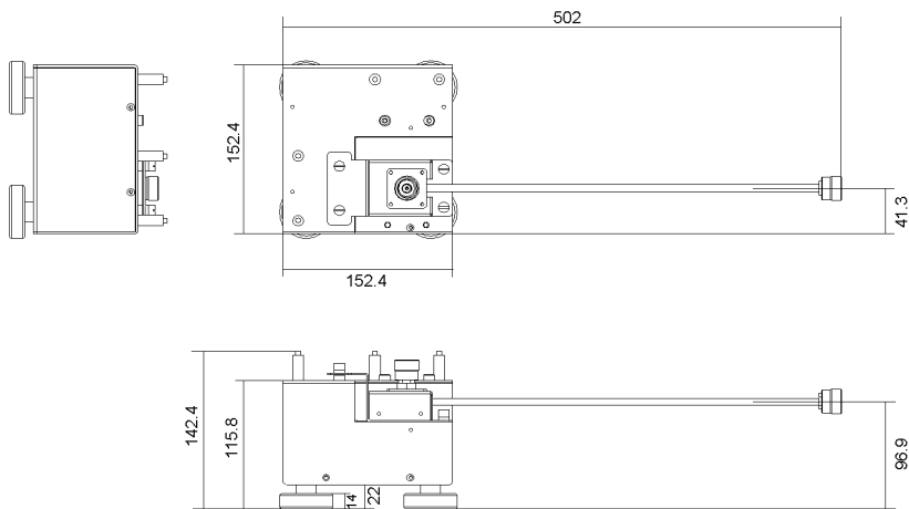
Figure 11. Option E4991A-007 test head dimensions (in millimeters, nominal)
