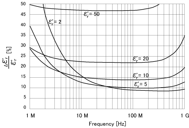
Figure 36. Permittivity accuracy \frac{(\Delta\epsilon')}{\epsilon'} vs. frequency (at t = 0.3 mm, typical)
