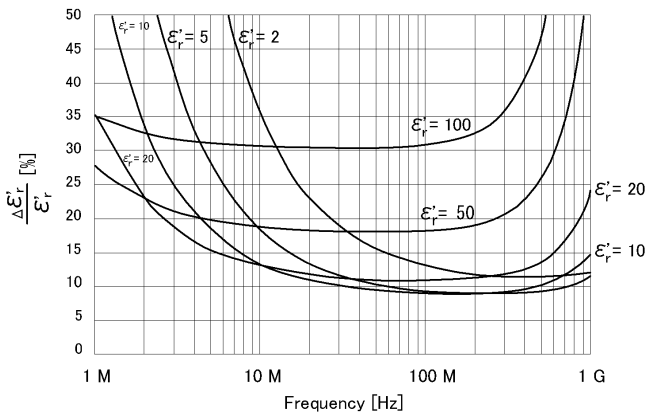
Figure 37. Permittivity accuracy \frac{(\Delta\epsilon')}{\epsilon'} vs. frequency (at t = 1 mm, typical)
