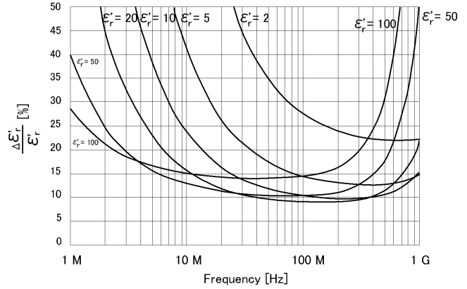
Figure 38. Permittivity accuracy \frac{(\Delta\epsilon')}{\epsilon'} vs. frequency (at t = 3 mm, typical)
