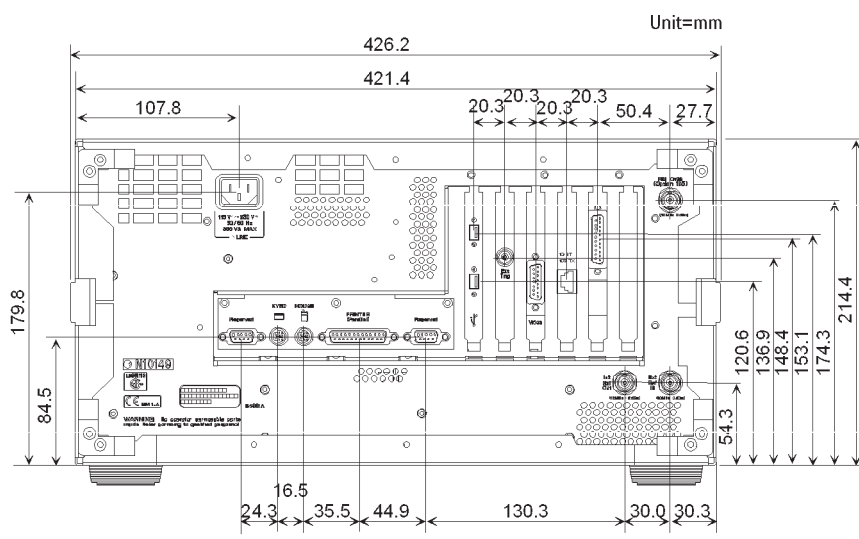
Figure 8. Main unit dimensions (rear view, in millimeters, nominal)
