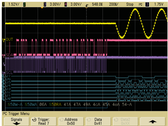
Figure 5. The MSO option lets you see the complex interactions among your signals on up to 20 channels at the same time.
